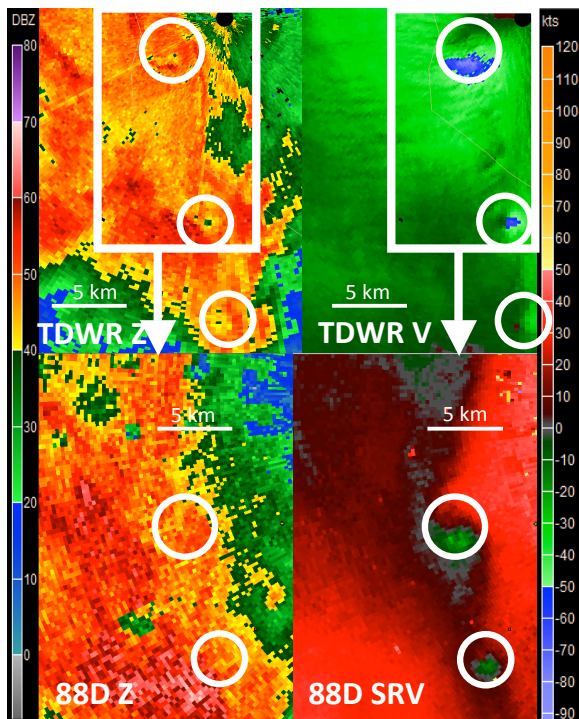
Figure 1. (Top) Terminal Doppler Weather Radar (TDWR) view at close range of a series of misocyclone circulations (circled) in a quasilinear convective system at various stages of development. (Bottom) WSR-88D view of the northern two circulations, also at close range but from a different viewing angle.
